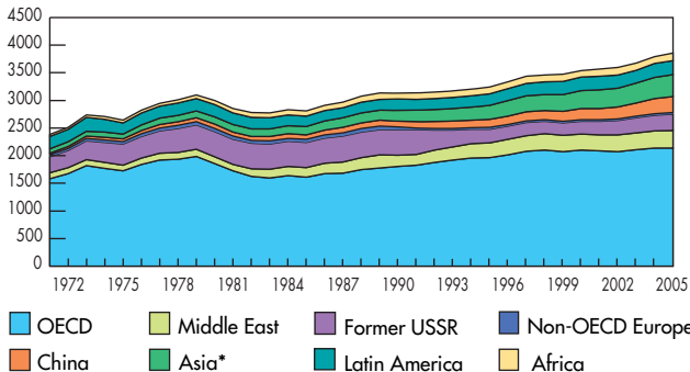
Evolution from 1971 to 2005 of World Refinery Throughput by Region (Mt)
