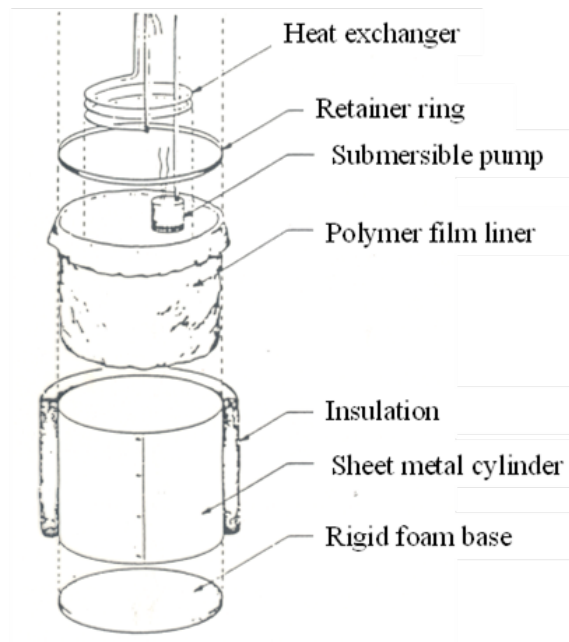
Figure 43. Schematic of low-cost polymer film membrane tank with immersed load-side HX and solar-loop pump
