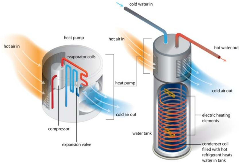
Figure 6. Schematic of HPWH technology
