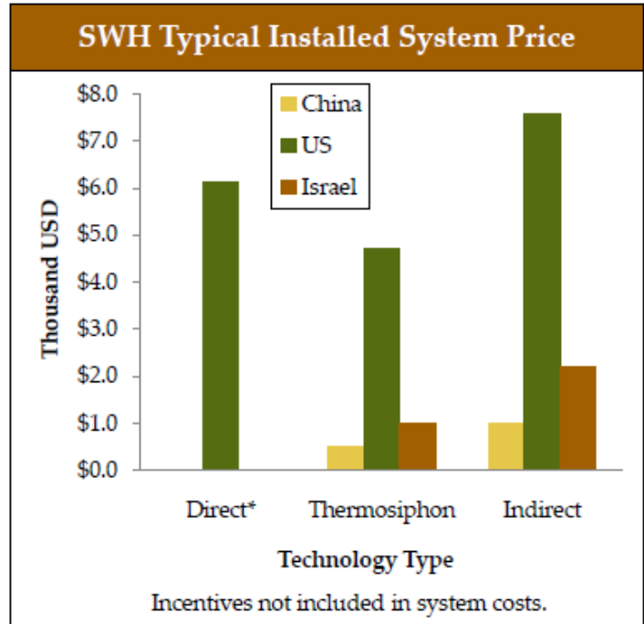
Figure 33. Installed SWH system costs 5
