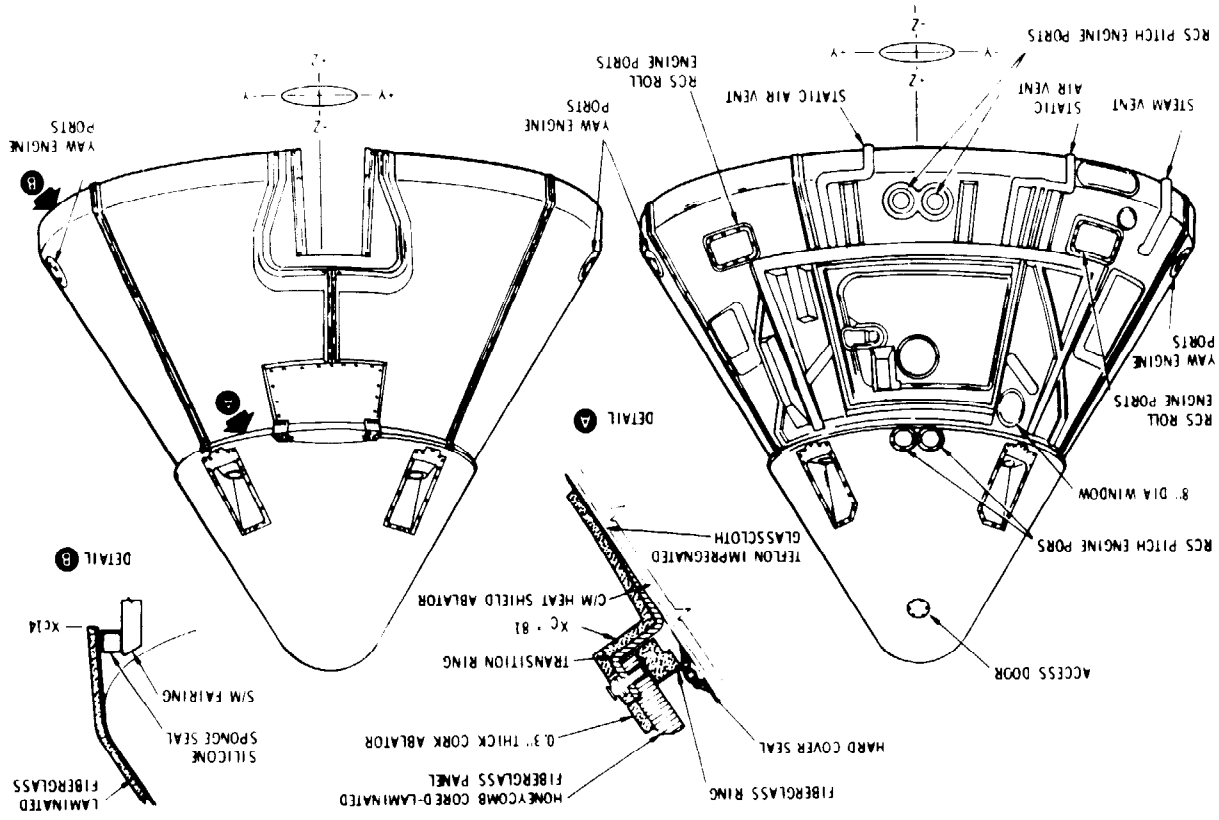
Figure A1-3.- Boost protective cover.
