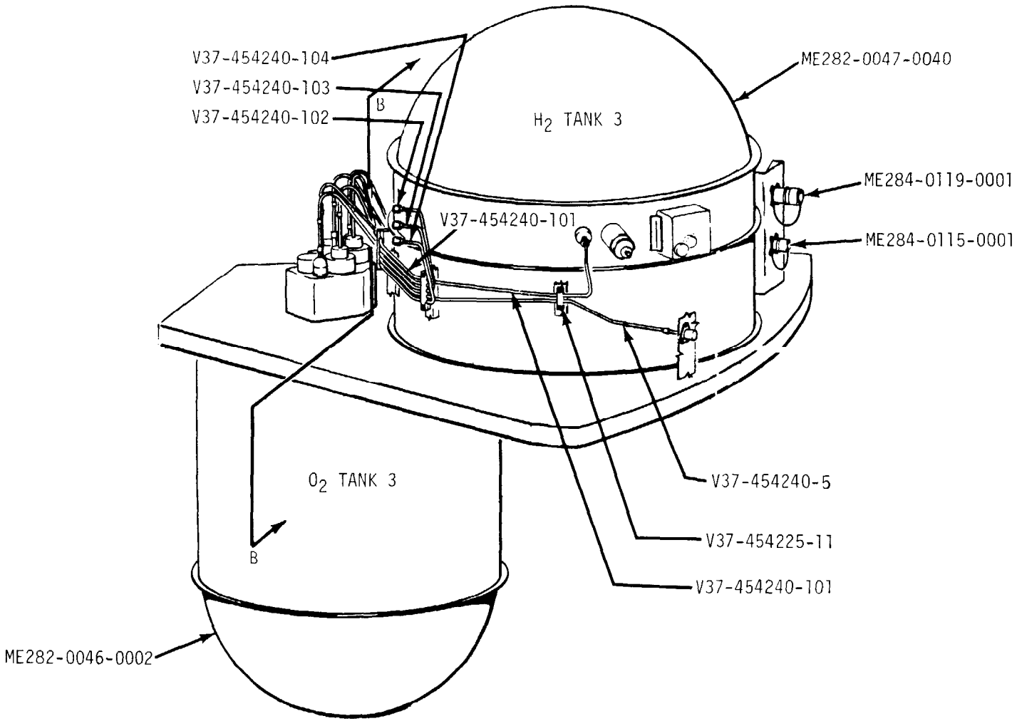
HYDROGEN/OXYGEN TANK SHELF MODULE - SECTOR I (SIDE VIEW - BEAM 6 SIDE)
