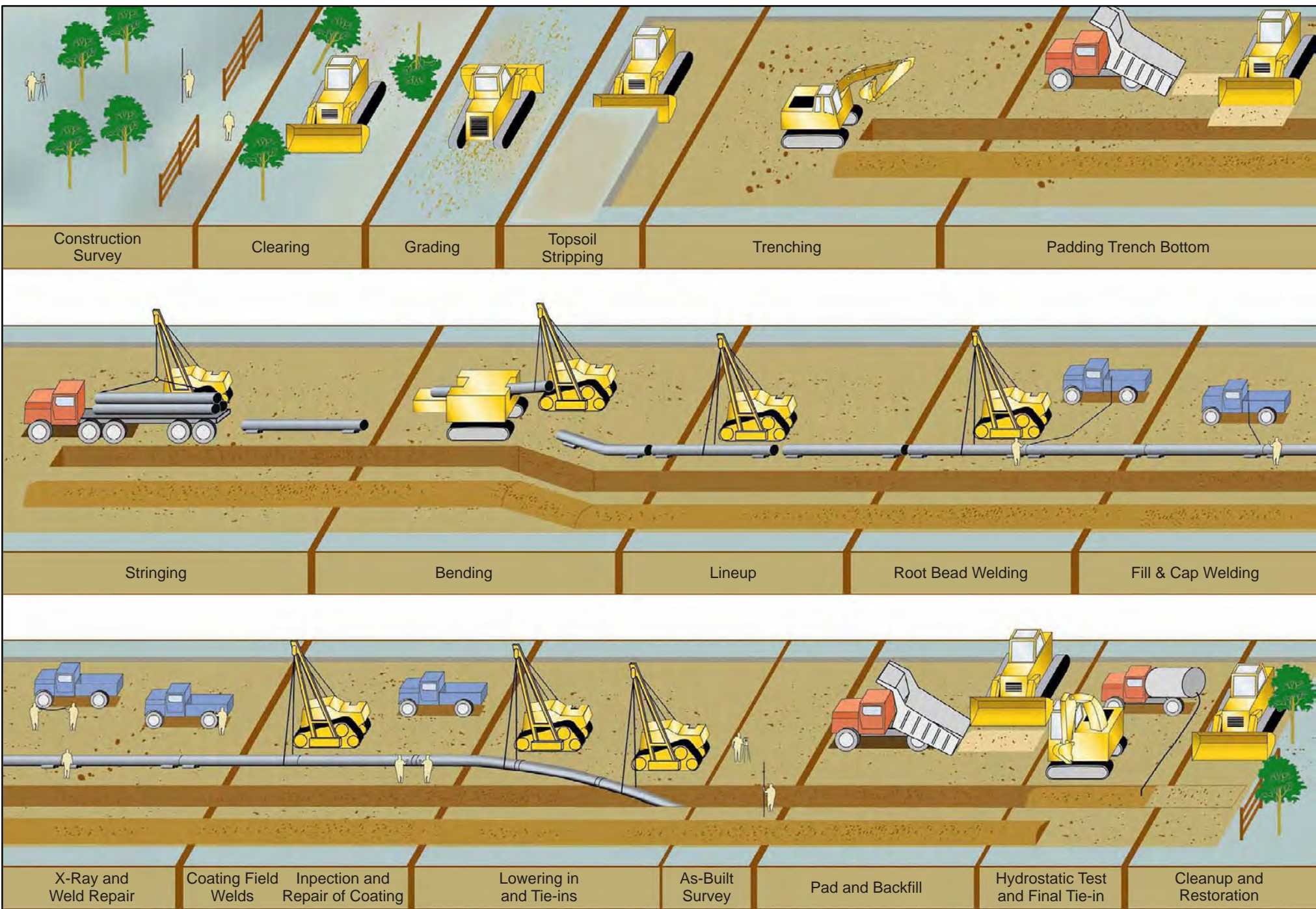
Figure 2.3.2-2 Typical Pipeline Construction Sequence
