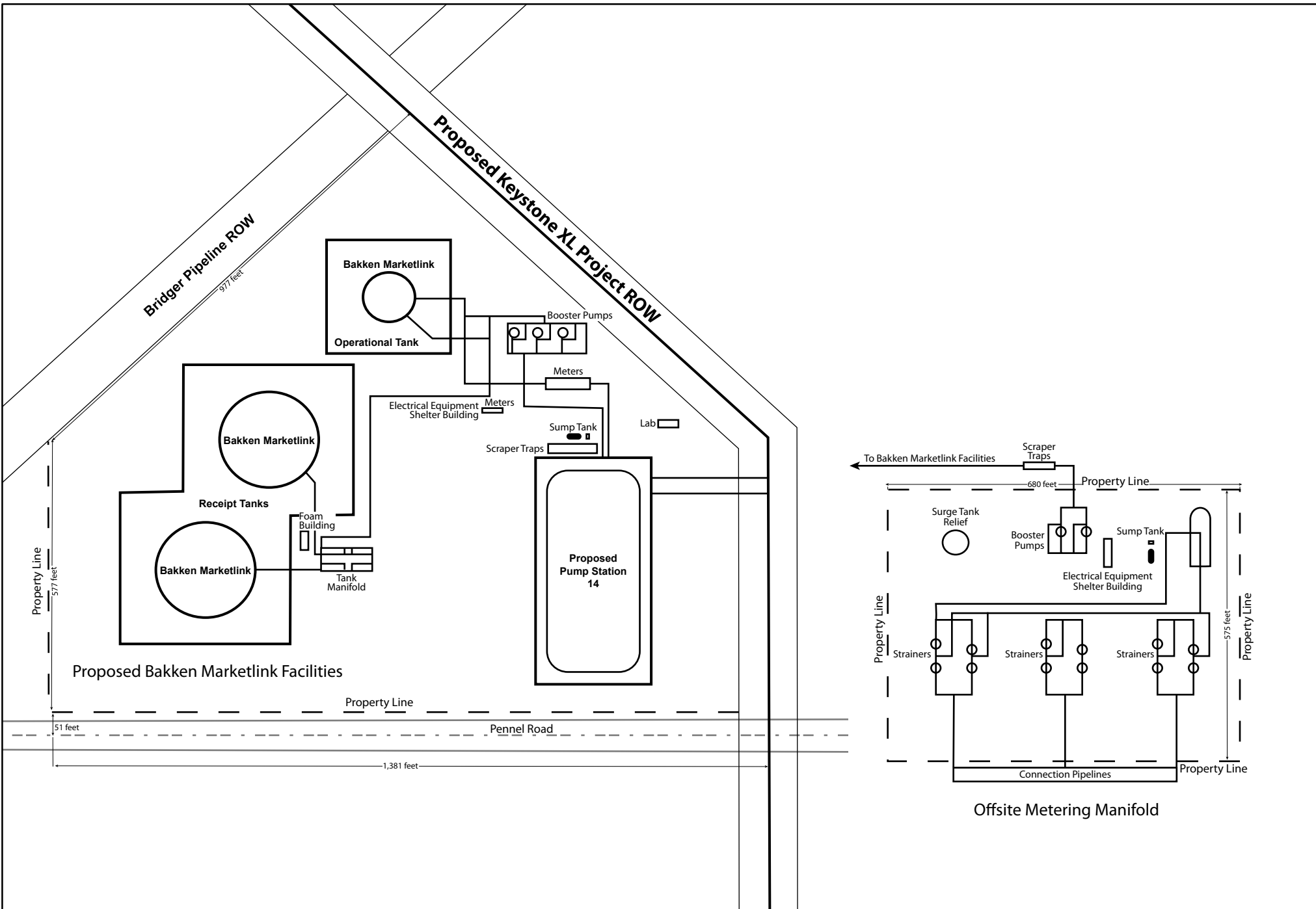
Figure 2.5.3-2 Plot Plan for Planned Bakken Marketlink Facilities near Baker, Montana
