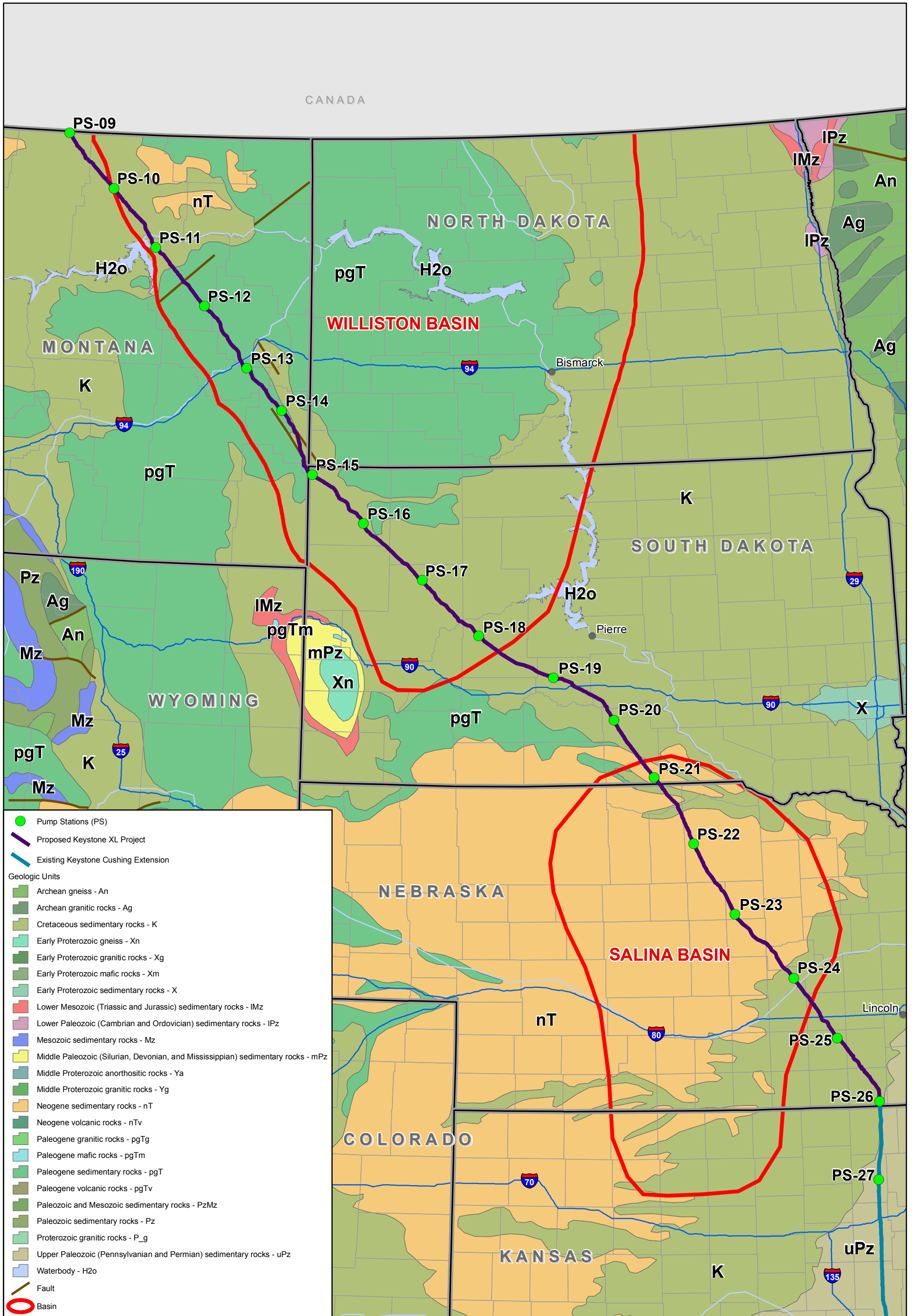
Figure 3.1.1-1 General Geology Steele City Segment
