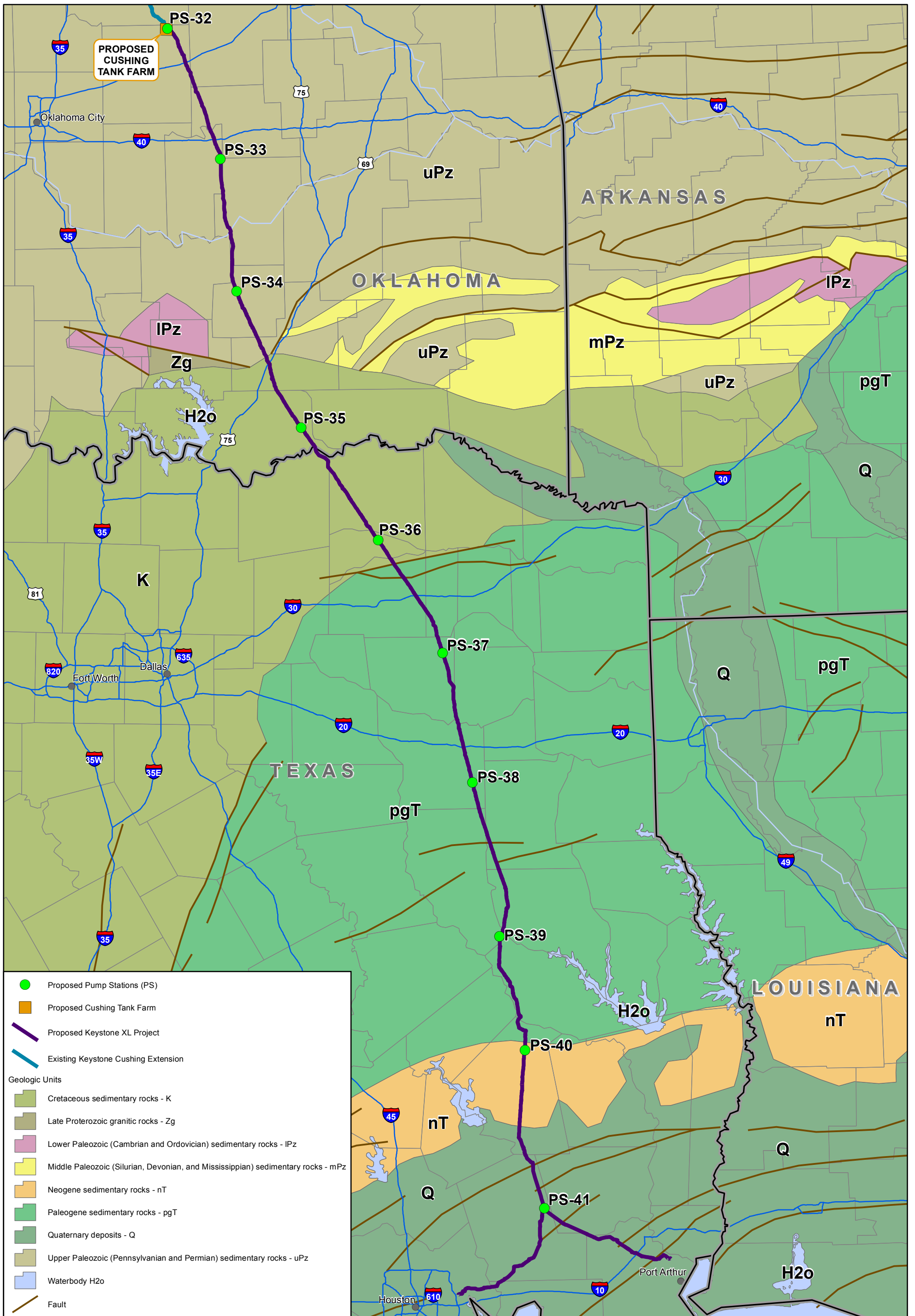
Figure 3.1.1-2 General Geology Gulf Coast Segment
