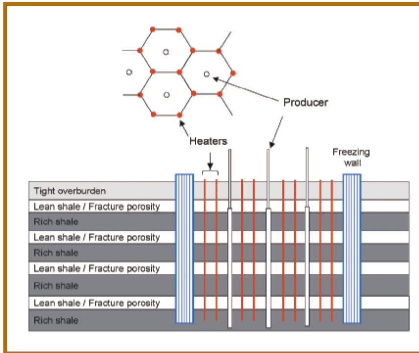
Figure 4-14. Shell In situ Conversion Process.
