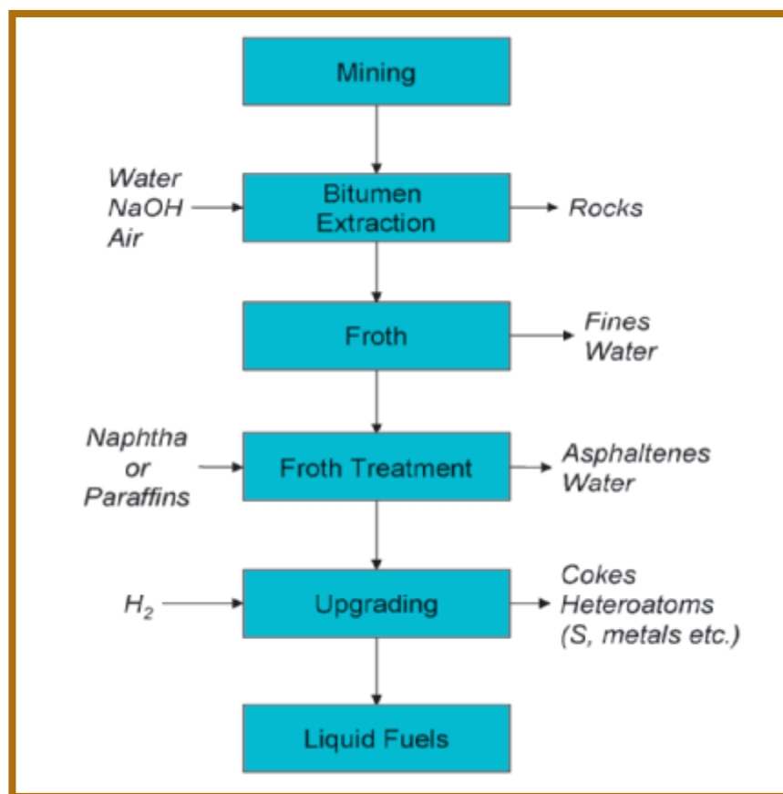
Figure 4-5. Schematic diagram of a water-based bitumen recovery process.
