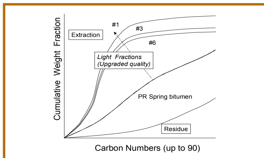
Figure 5-3. Conceptual simulated distillation curves for the extract, bitumen and the residue after supercritical extraction.
