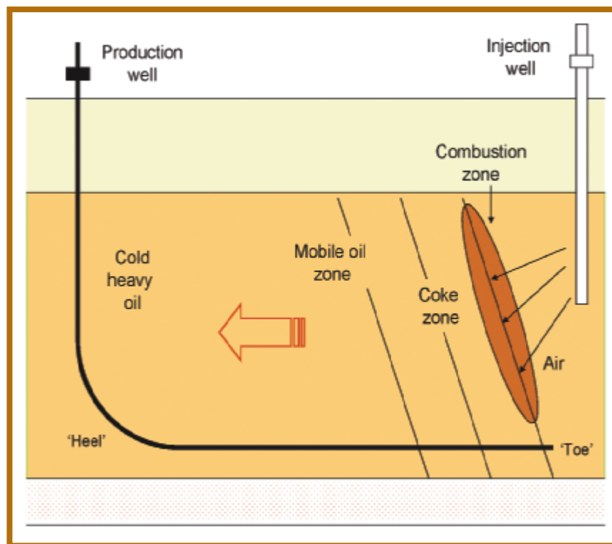
Figure 4-9. Schematic of the THAI Process.
