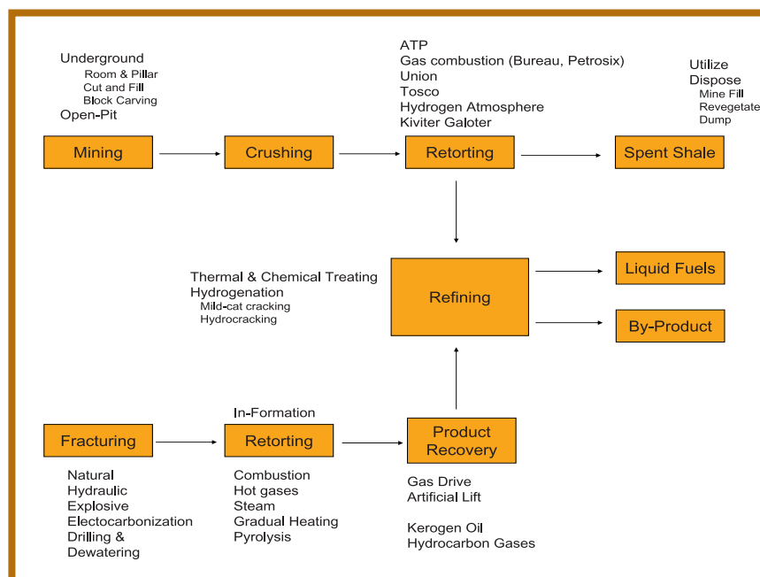
Figure 4-10. Generalized processes for conversion of shale to fuels and byproducts.
