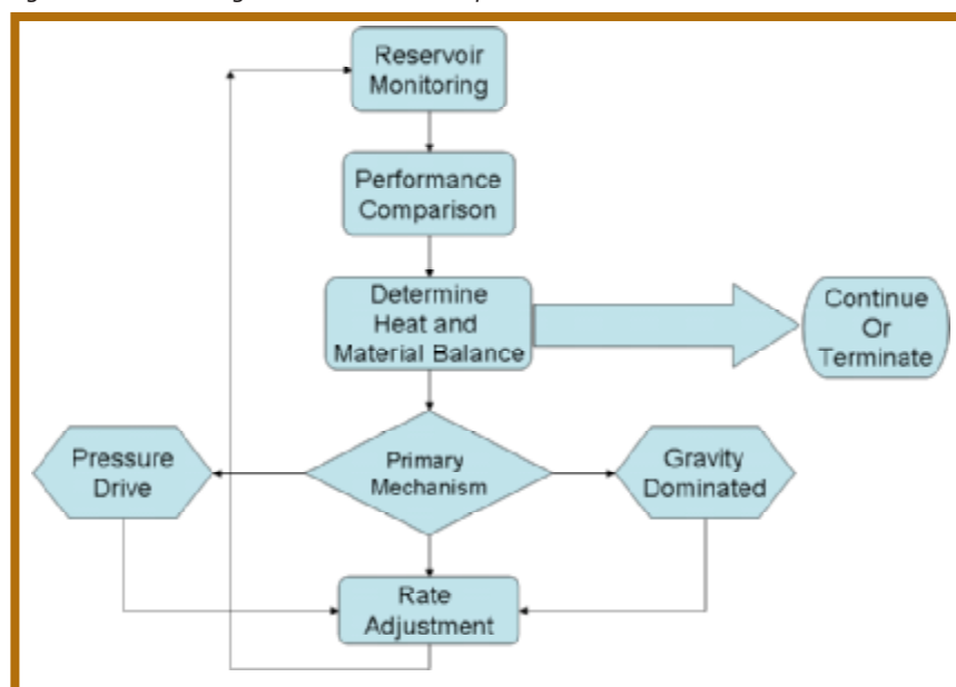
Figure 4-3. Heat management in a steamflood process.
