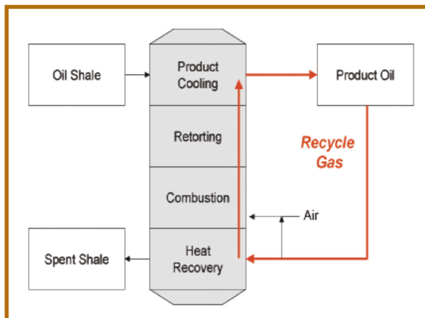
Figure 4-12. Gas combustion retorting process.
