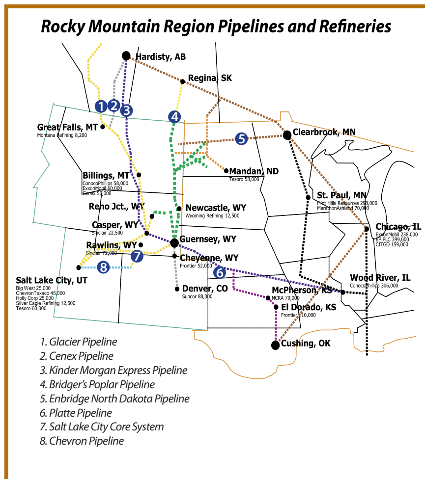
Figure 6-6. Crude oil pipelines and refineries, with capacities in barrels per day, in the Rocky Mountains and the Midwest.
