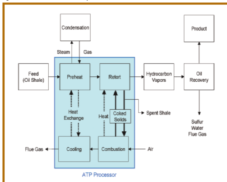
Figure 4-13. Alberta Taciuk Process system.
