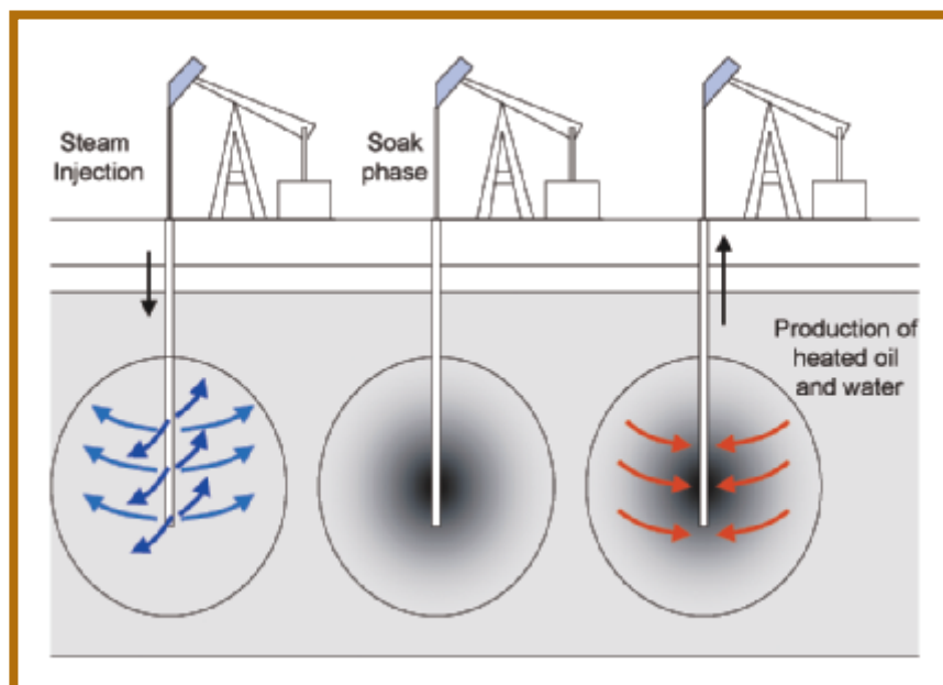
Figure 4-7. Schematic of a cyclic steam stimulation process showing injection, soak and production.
