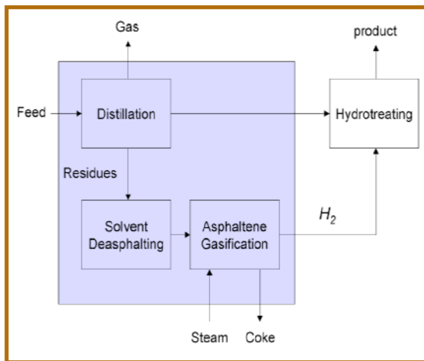
Figure 5-1. Combination of technologies to reduce dependence of upgrading on natural gas.
