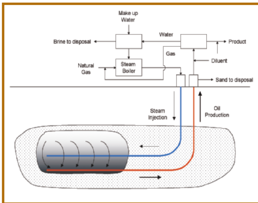
Figure 4-8. Illustration of the SAGD process including the horizontal injector, the horizontal producer, and some surface facilities.
