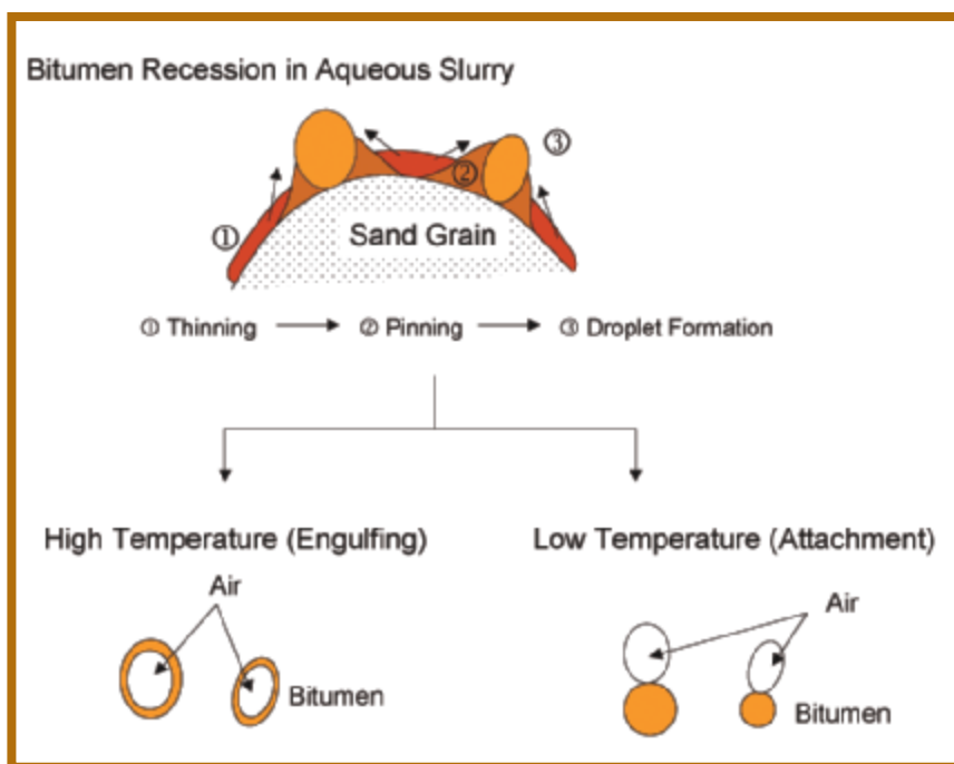
Figure 4-6. Bitumen liberation and aeration in water-based extraction process.
