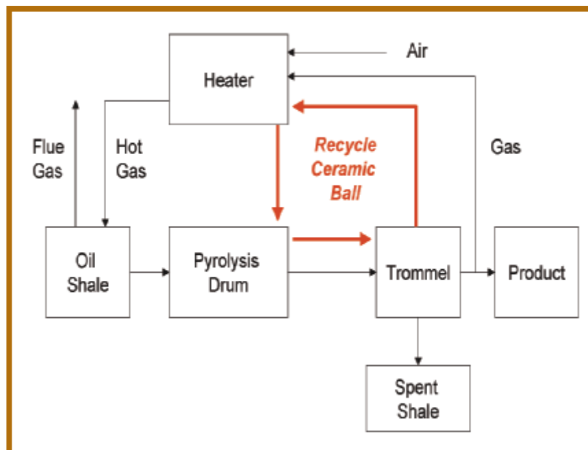
Figure 4-11. TOSCO II process.
