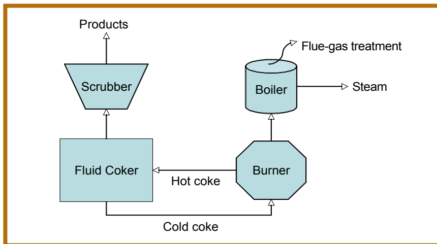
Figure 5-2. Schematic of a fluid coker.
