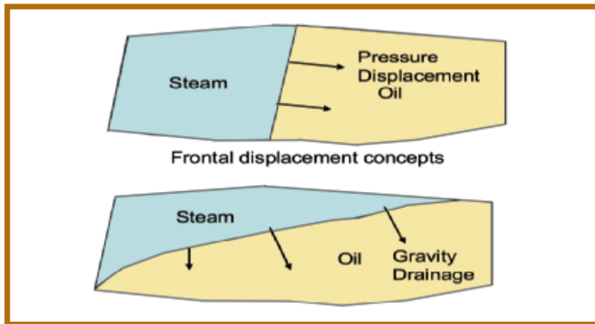
Figure 4-4. Evolution of steamflood theory from a pressure displacement process to a gravity drainage process.
