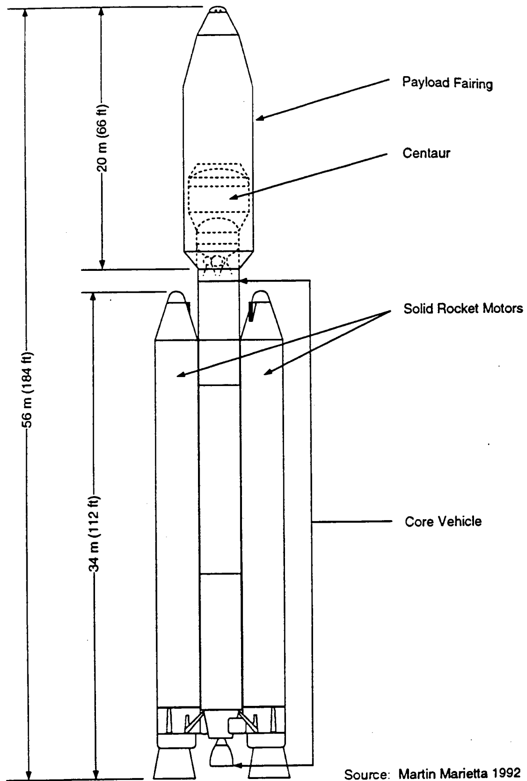
Figure 2-4 Diagram of the Titan IV (SRMU)/Centaur Launch Vehicle
