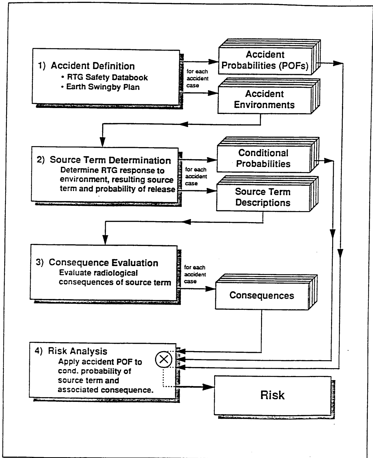
Figure 4-1 Overview: Basic Elements in the Nuclear Launch Safety Risk Analysis Process
