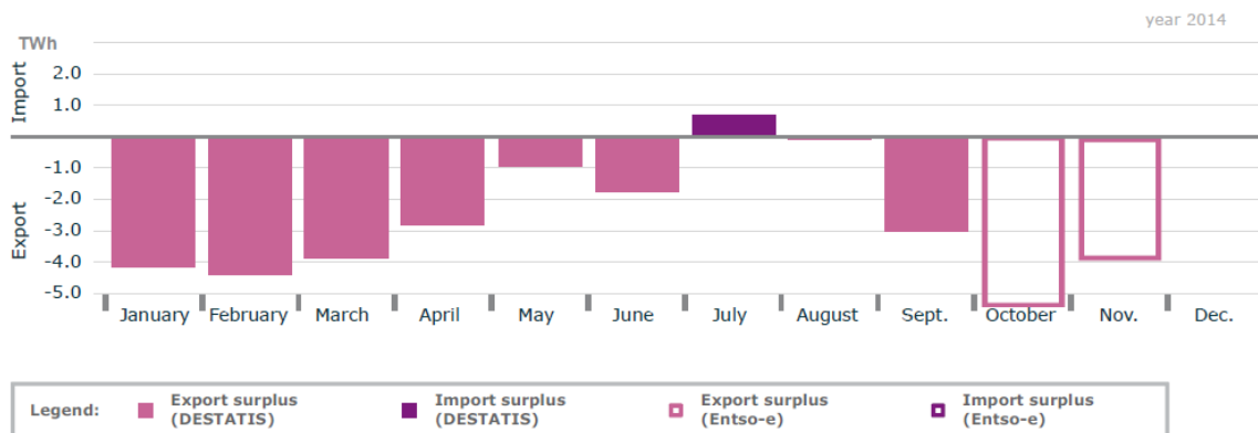
Figure 18: Monthly power export and import balances in 2014. [ISE4]
