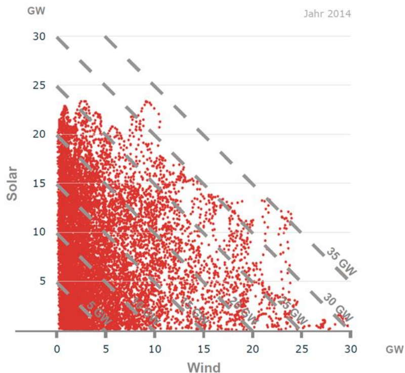
Figure 27: Average hourly amount of solar and wind energy fed into the grid in 2014 [ISE4].
