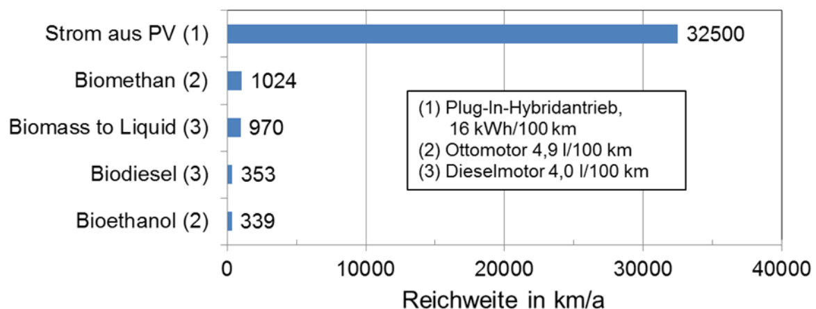
Figure 31: Vehicle range for an annual yield of 1 a = 100 m 2 of energy crops (2,3) or 40 m 2 of elevated PV modules constructed on 100 m 2 on flat, open ground, Sources: Photon, April 2007 (1) and Fachagentur Nachwachsende Rohstoffe (2), (3).
