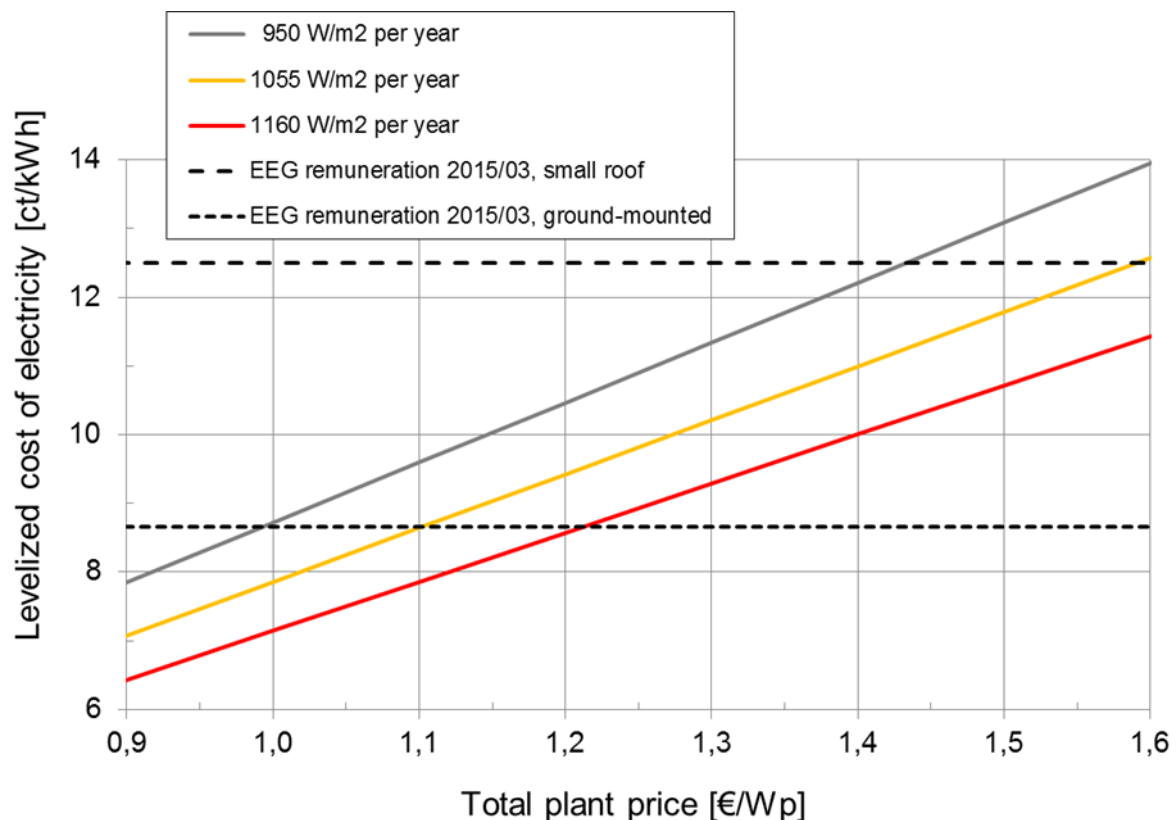
Figure 19: Rough estimate of levelized cost of electricity (LCOE) for PV power plants at different annual irradiances
