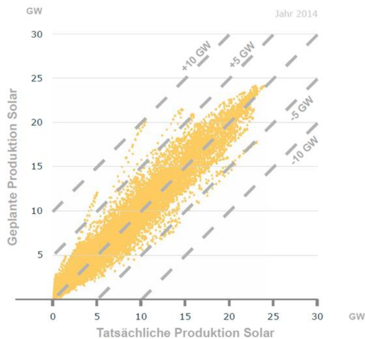
Figure 26: Actual and predicted hourly generation of power in 2014 [ISE4].
