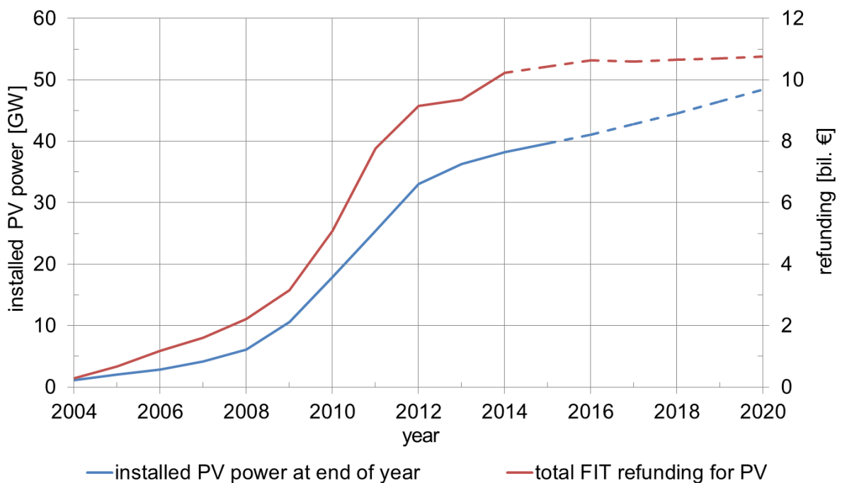
Figure 6: PV expansion and total feed-in tariff, (Data from [BMWi1]; Annual figures and prognosis of German grid operators [ÜNB]).
