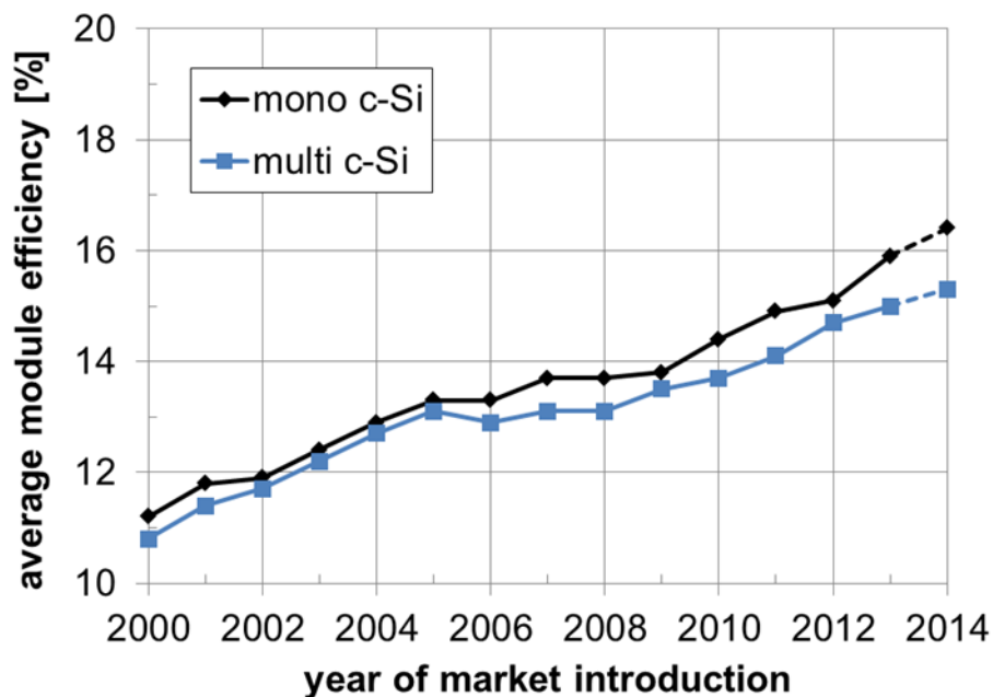
Figure 30: Development of the mean efficiency of PV modules, based on mono and multi-crystalline solar cells, according to year of market introduction. Data from Photon International 2014-02.
