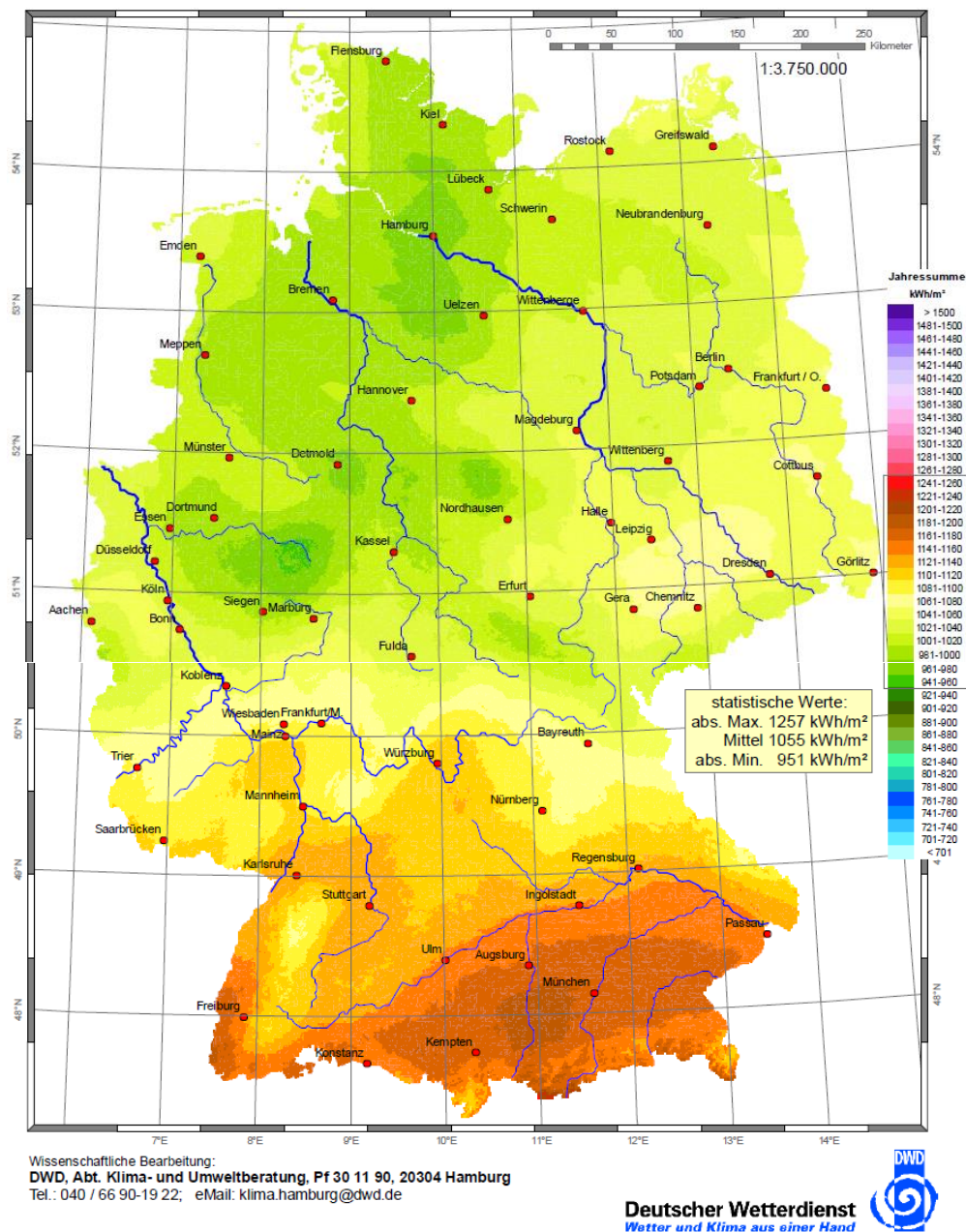
Figure 33: Horizontal annual global irradiation in Germany averaged over 1981-2010
