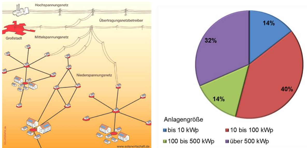
Figure 25: Left: Schema of PV power feed-in [BSW], Right: Installed PV power categorized by system size (as of Dec. 2015) (Data up to 2008 from transmission system operators (TSO), 2009: Bundesnetzagentur (German Federal Network Agency); Data compiled by PSE/Fraunhofer ISE.
