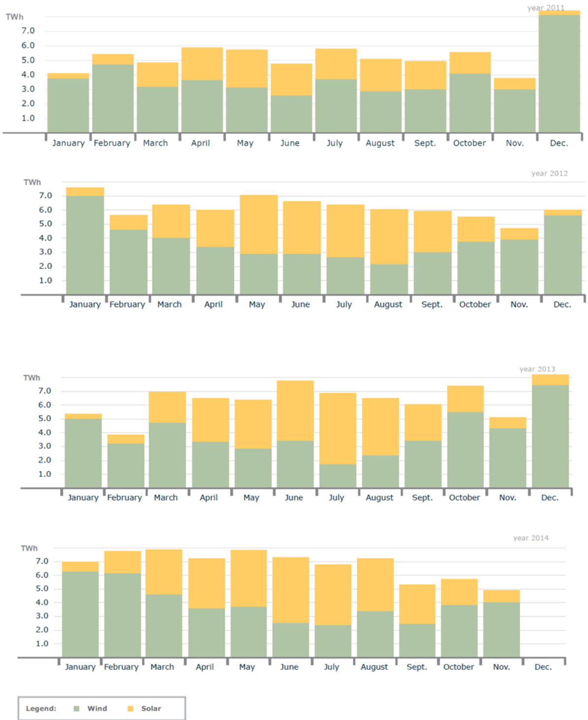
Figure 28: Monthly production of PV and wind power for 2011 - 2014 [ISE4].
