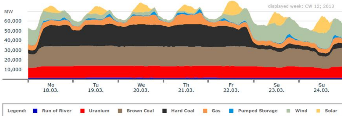
Figure 29: Example showing course of electricity trading price, conventional and renewable electricity in the 12th calendar week (March 2013)
