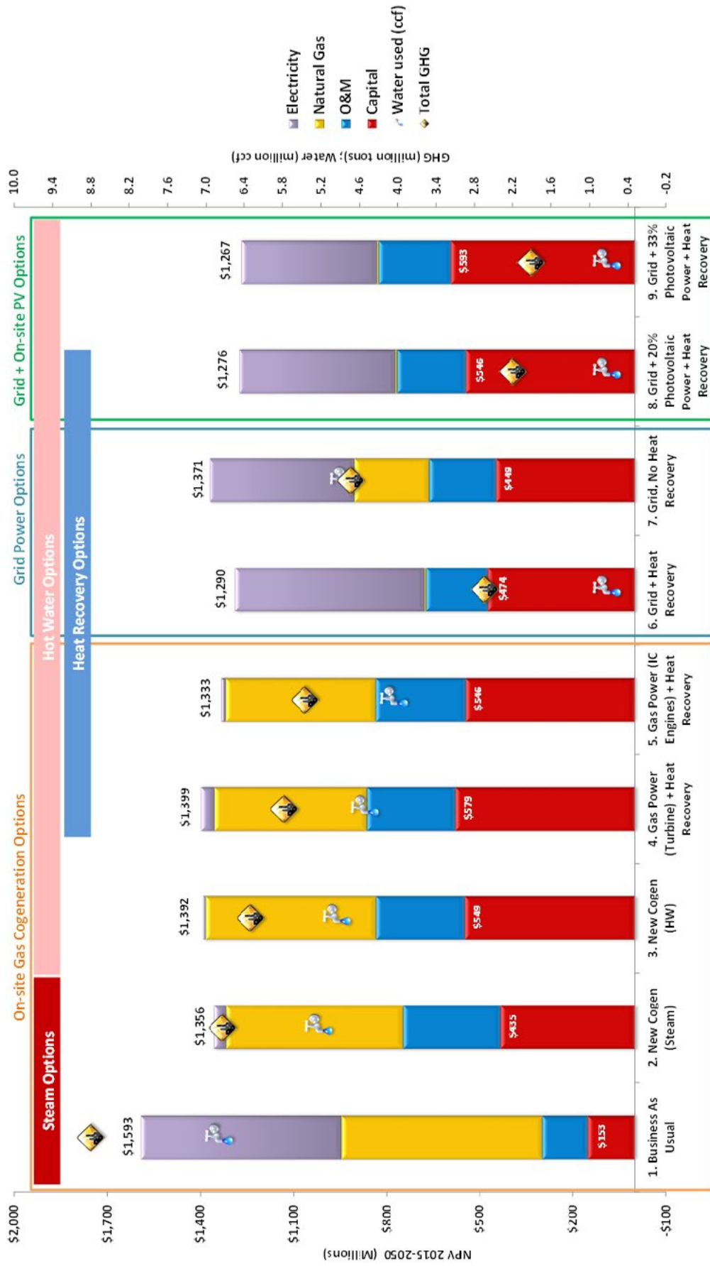
FIGURE 6-5 COMPARATIVE COST, GHG, AND WATER USE OF ENERGY SUPPLY OPTIONS
