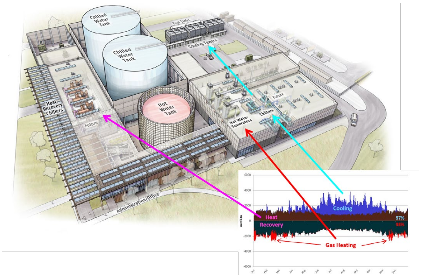
FIGURE 0-2 HEAT RECOVERY POTENTIAL AT STANFORD
